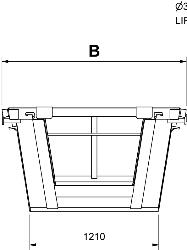
DOOR END VIEW
